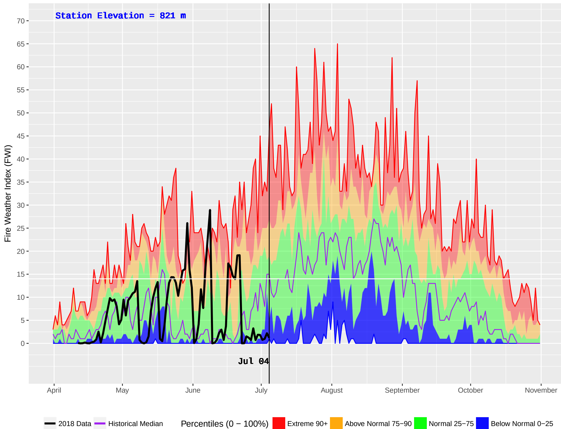
AKOKLI CREEK (838) : Historical (2003–2016) and Current (2018) Noon Fire Weather Index (FWI)
